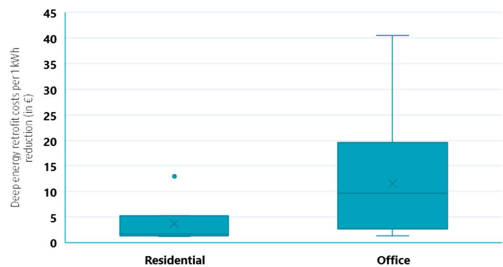
Figure 9 | Boxplot of costs to reduce energy consumption for residential and office buildings by 1 kWh/m²
