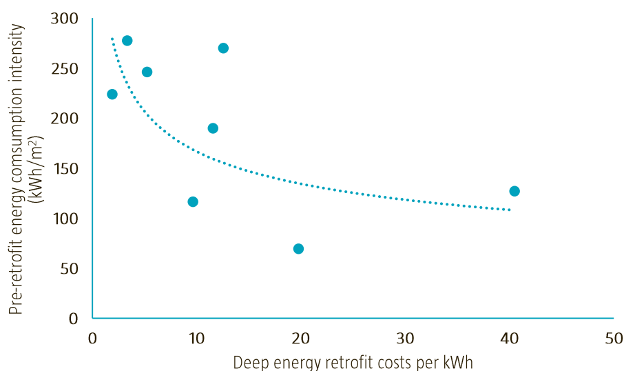
Figure 8 | Relation between the office buildings' pre-retrofit energy consumption intensity and the deep energy retrofit costs per kWh/m 2 reduction
