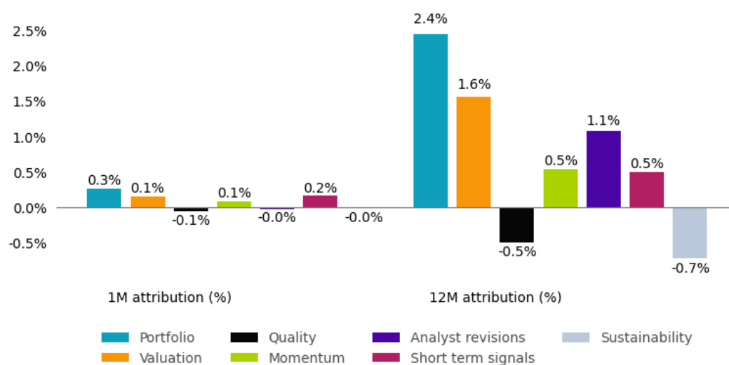
Figure 1 – Factor attribution
