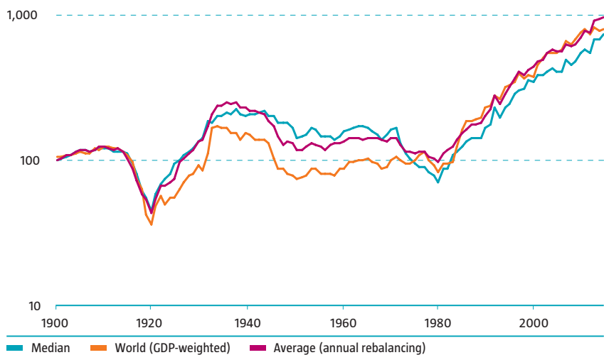
Figure 1.2: Real return index for global bonds with different weighting methods
